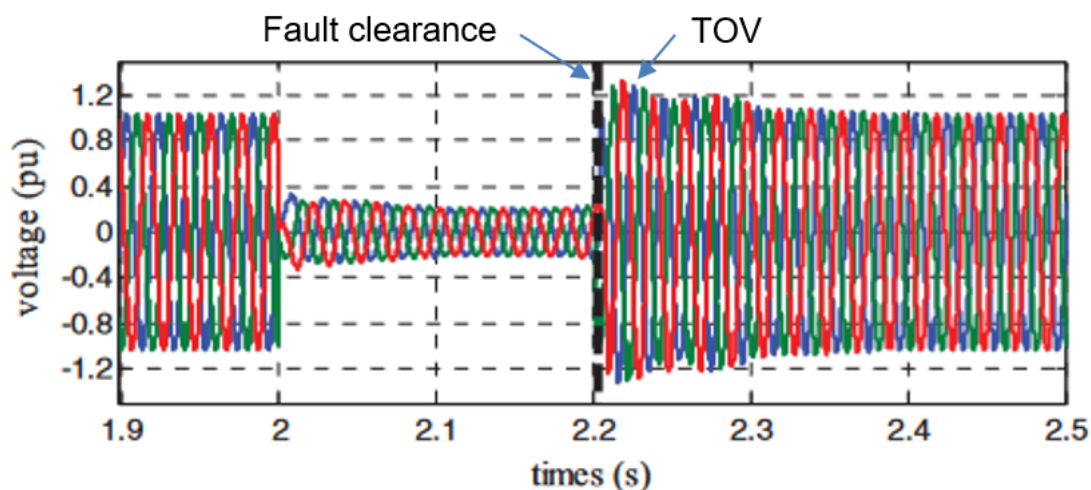
Figure D.10: Temporary over voltage
