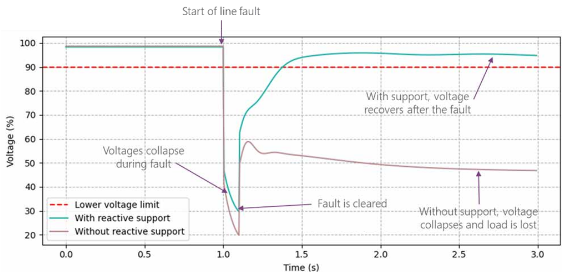
Figure D.9: Bus Voltage with and without reactive support
