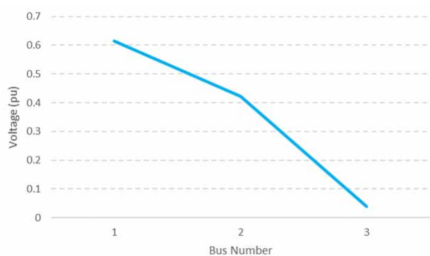
Figure D.7: Bus voltages during fault, with reactive current injection
