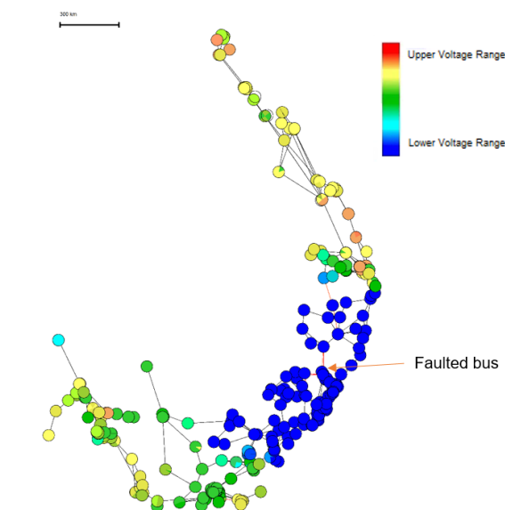
Figure D.6: Transmission bus voltages during fault
