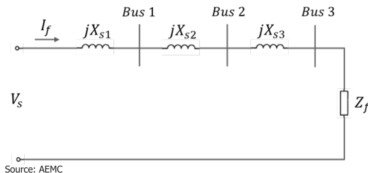
Figure D.3: Simplified equivalent circuit for a short circuit, with multiple buses
